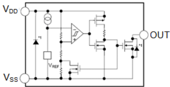
NMOS open-drain
